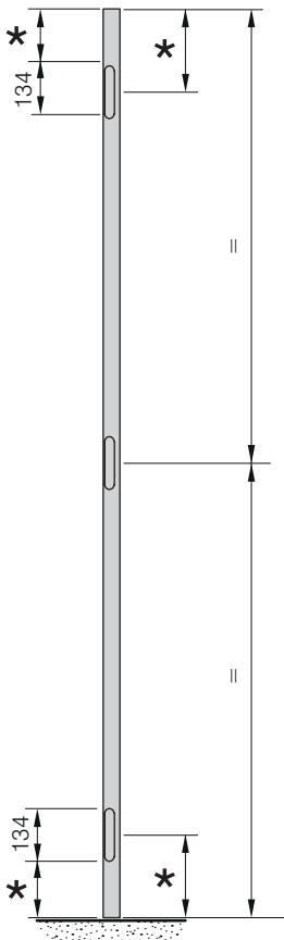
Jamb with 3 hinges flush with the ceiling version up to h. 2300
