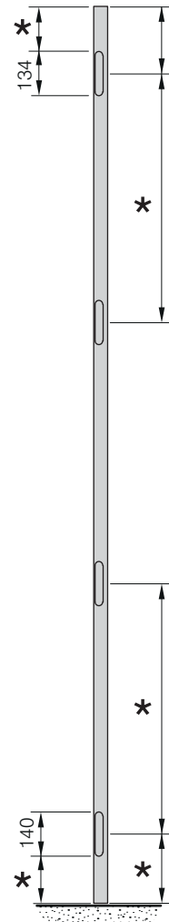
Jamb with 4 hinges flush with the ceiling version up to h. 3000
