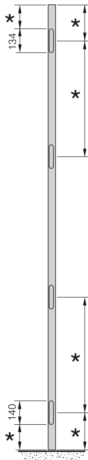
Jamb with 4 hinges flush with the ceiling version up to h. 2500
